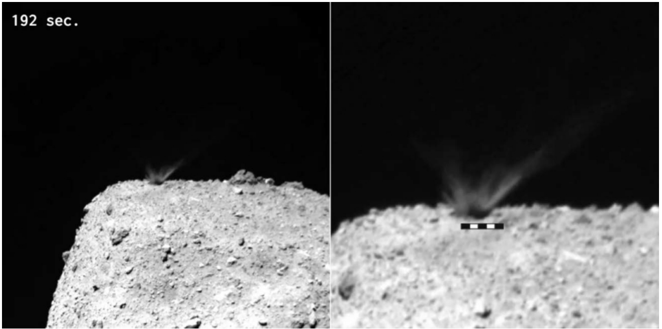
Figure 1: DCAM3 observations of the rocky surface of asteroid Ryugu at 192 seconds. ©Arakawa et al., 2020
